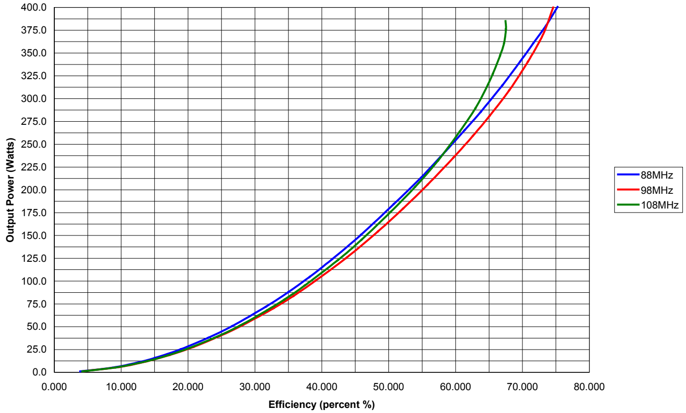
Efficiency Vs Output Power @ 48VDC; Class B 100 bias current SD2942
