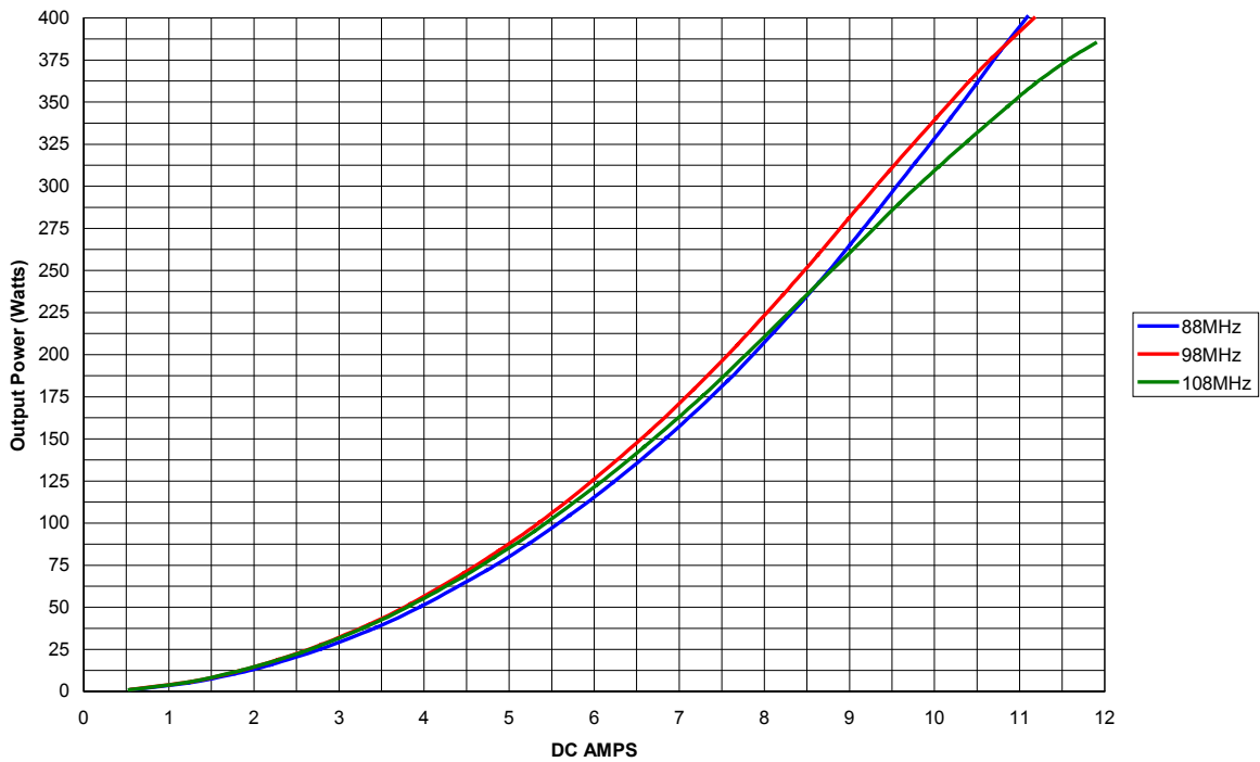
DC Amps Vs Output Power @ 48VDC; Class B 100ma bias current SD2942
