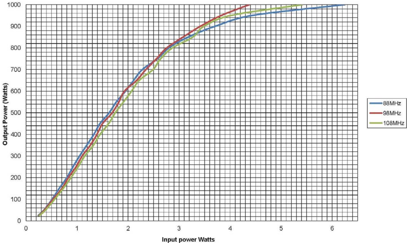
Input power & Output Power @ 50VDC; 100ma bias BLF188XR
