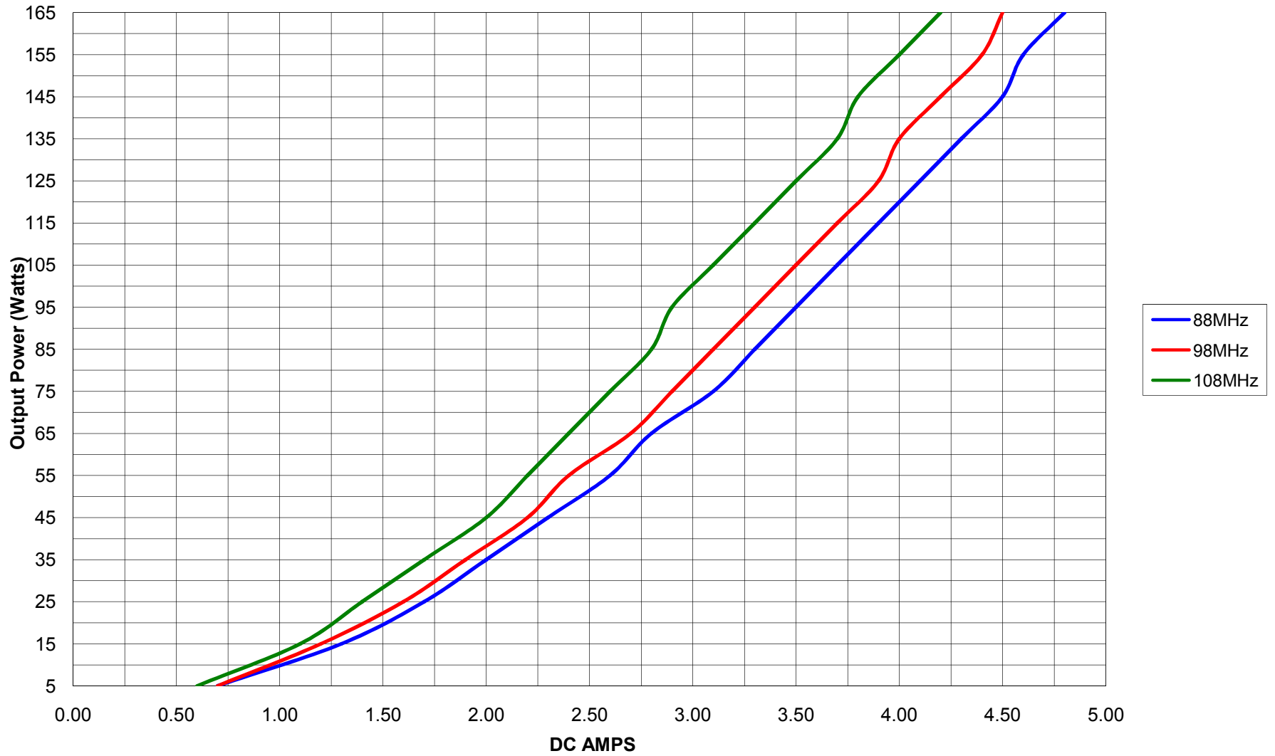
DC Amps Vs Output Power @ 48VDC; Class B 15ma bias current NXP BLF177
