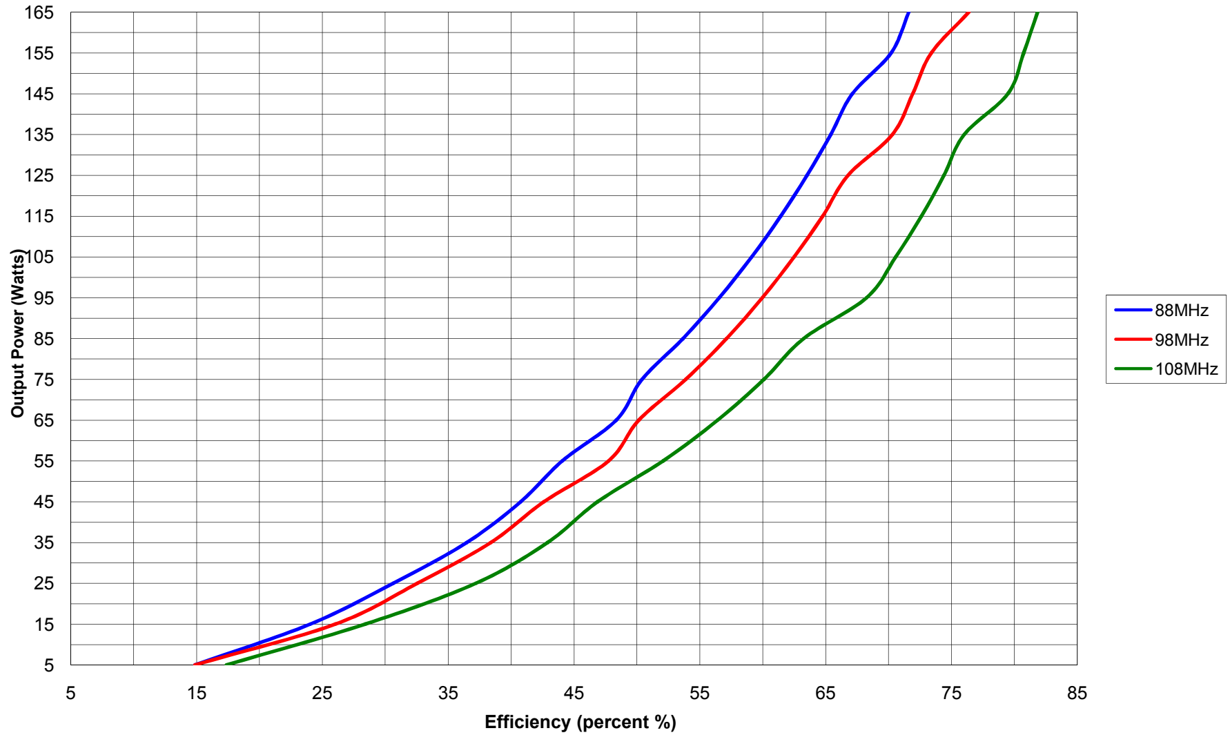
Efficiency Vs Output Power @ 48VDC; Class B 15ma bias current NXP BLF177
