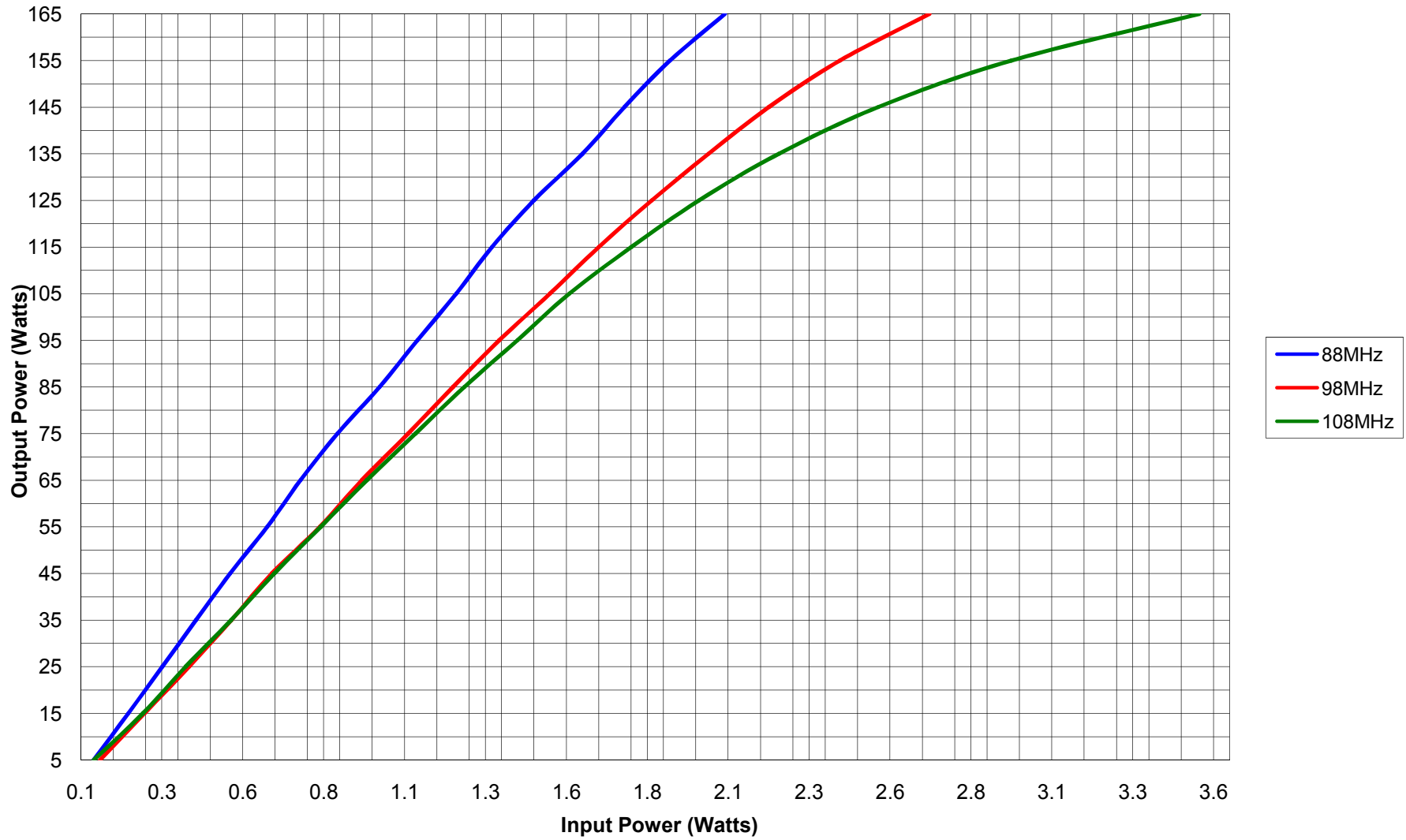
Input Power Vs Output Power @ 48VDC; Class B 15ma bias current NXP BLF177
